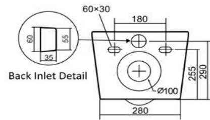
Back view
